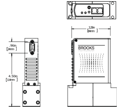
Electrical Connector SX Specific Dimensions
